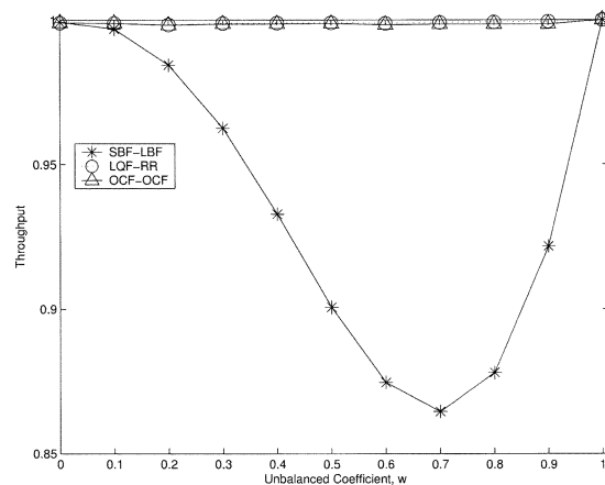
Fig. 4. Stability under nonuniform traffic, internal buffer = 1 cell.
