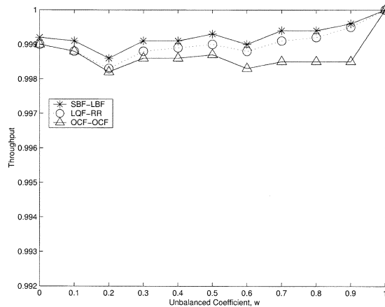
Fig. 5. Stability under unbalanced traffic and internal buffer = 8 cells.
