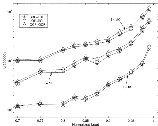
Fig. 3. The l -two norm vector under Bursty uniform traffic.
